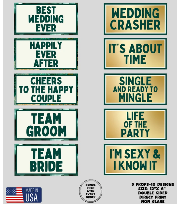
#29 – Wedding Bundle 3
